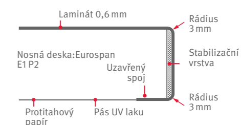
Model 300 / 3
